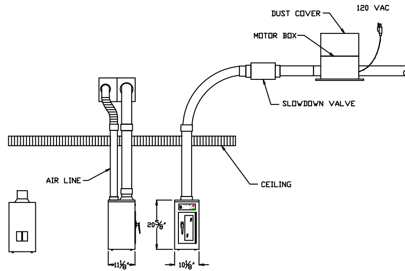
ALTERNATE INSTALLATION
