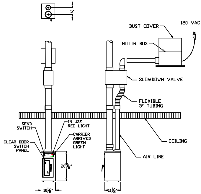
PREFERRED INSTALLATION
